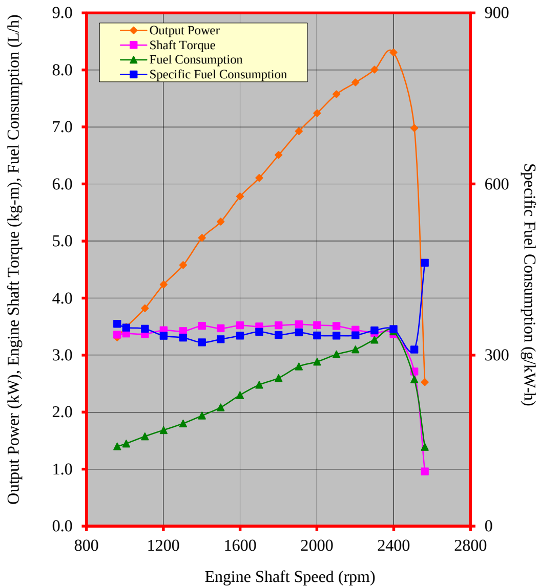
Figure 3. Performance characteristic curves of the PLATINUM PT110 KNM1100 diesel engine
