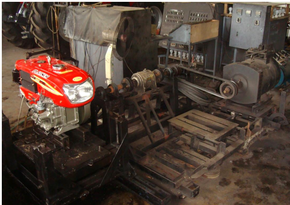
Figure 2. Test set-up of the PLATINUM PT110 KNM1100 Diesel Engine
