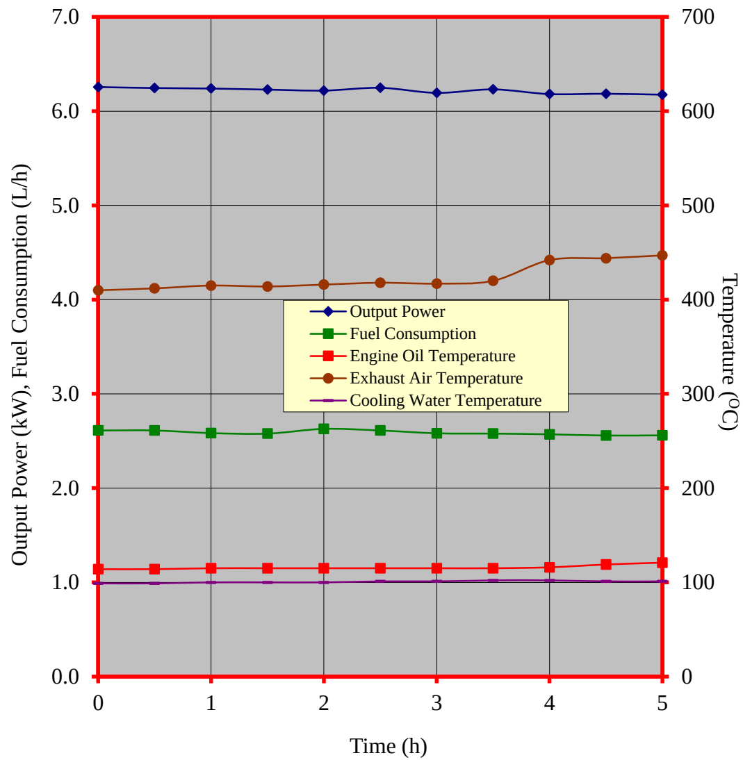
Figure 4. Performance characteristic curves during the continuous running test of the PLATINUM PT110 KNM1100 diesel engine
